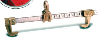
Beamer 2000 + Fits a Wide Variety of Beam Sizes from 3-1/2" to 14" Ratcheting End Piece Fast and Easy Installation VV1A-00102
